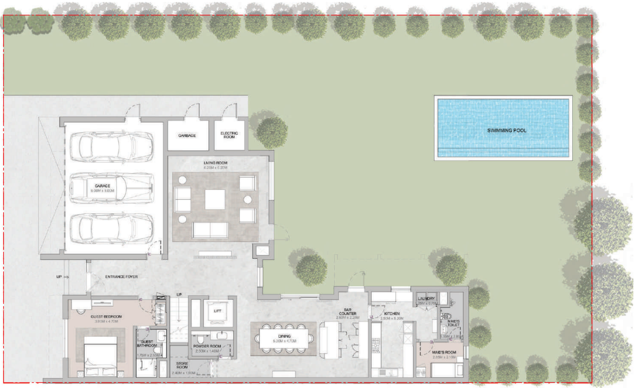
Ground Floor
